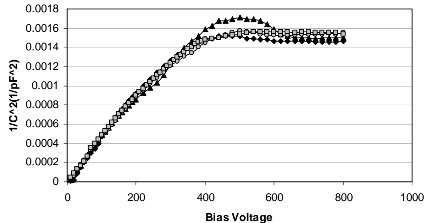
p-type MCz
