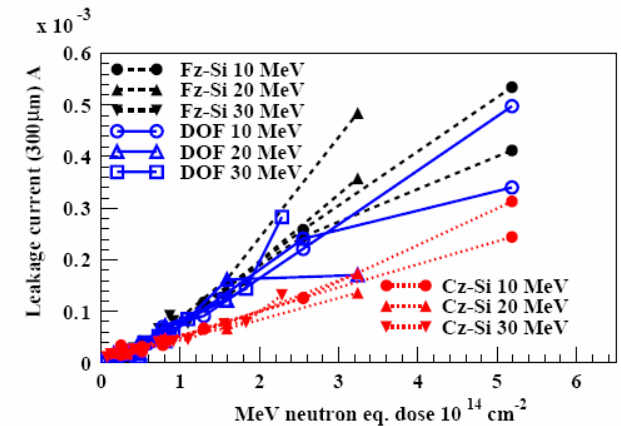
Fig. 2. Leakage current of oxygenated Fz-Si, Fz-Si and Cz-Si as a function of fluence.
